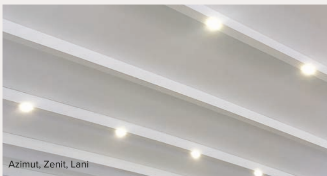
Azimet, Zenit
